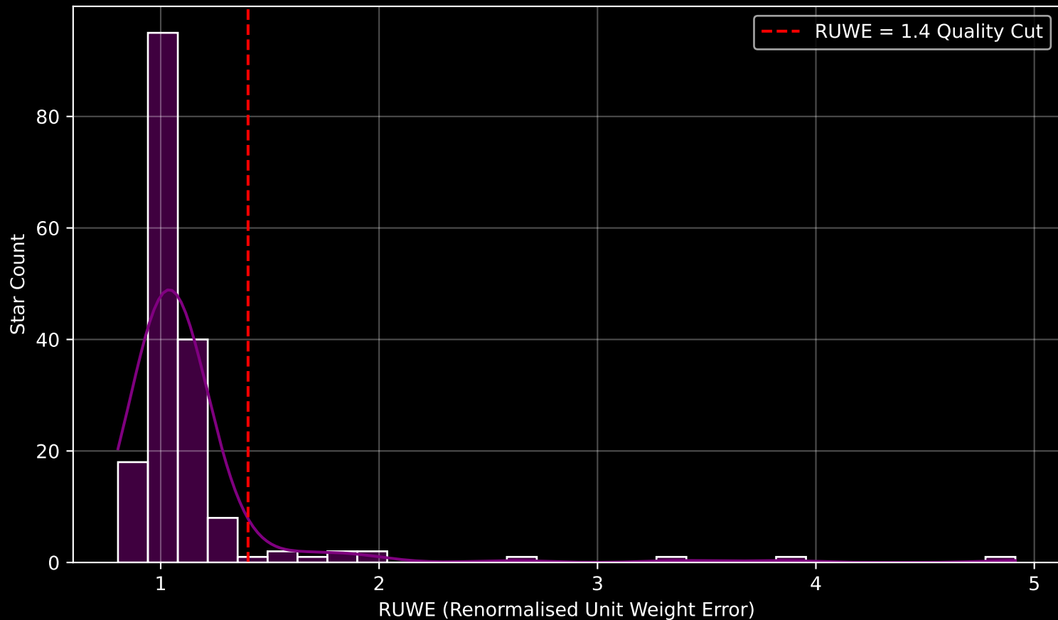
GAPOGEE DR17 Field [191-04] RUWE Distribution (n= 173)
