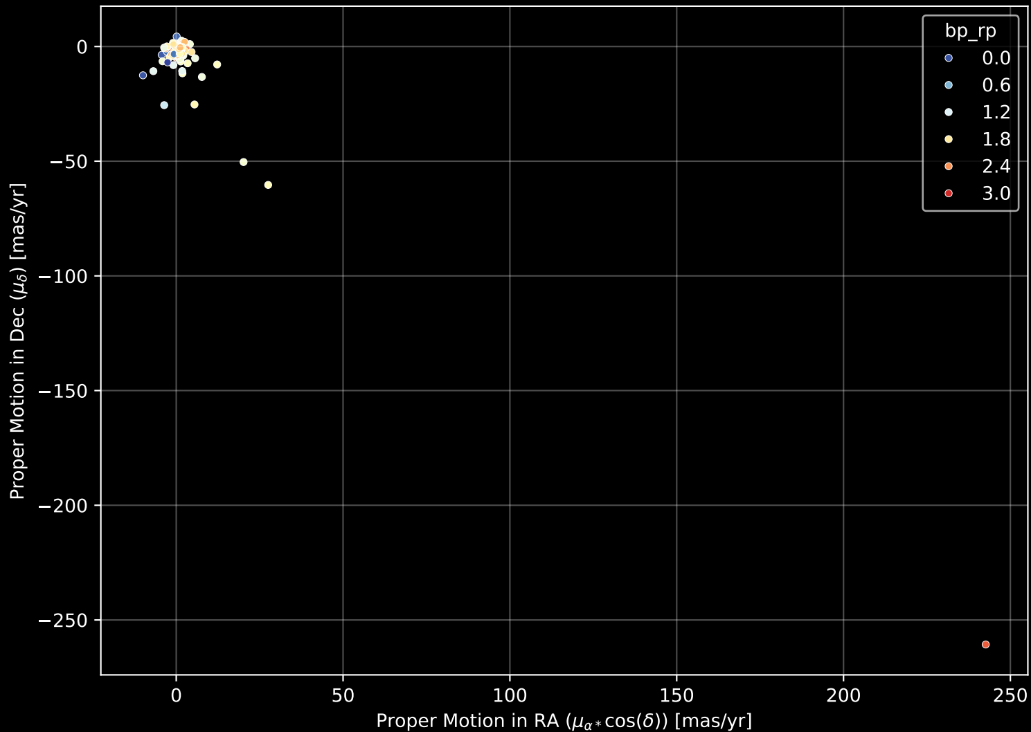
APOGEE DR17 Field: [191-04] Proper Motion Diagram (n= 176)
