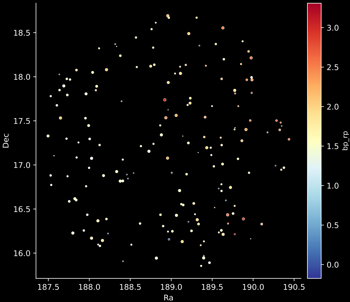
APOGEE DR17 Field: [191-04] Stars: 176
