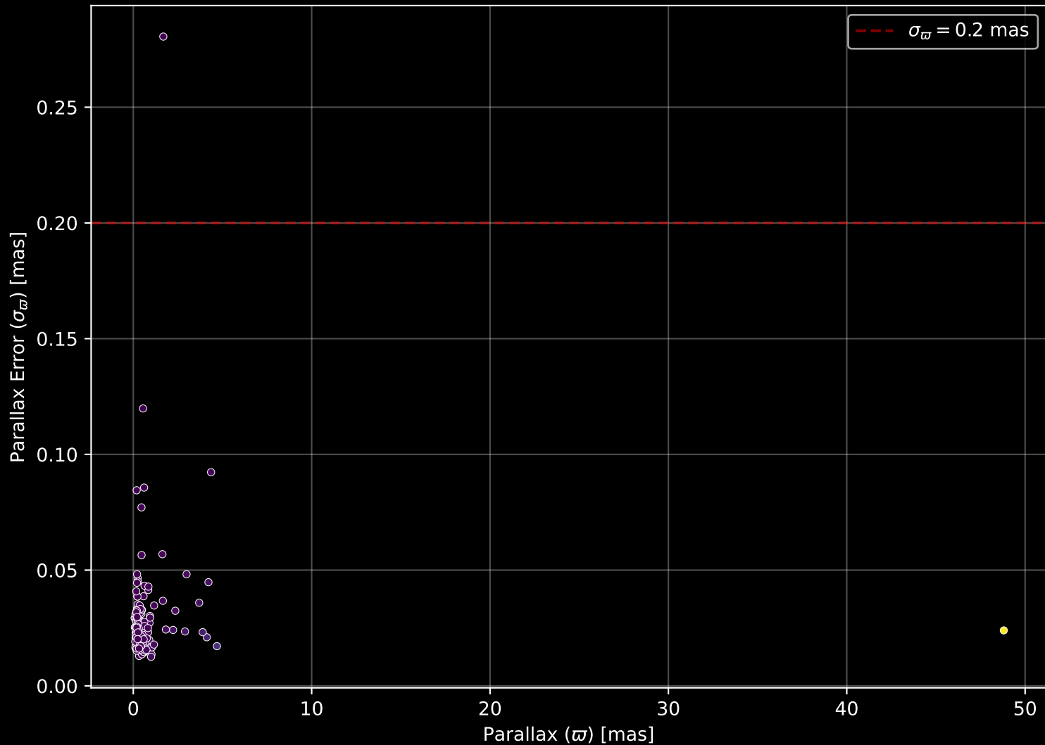
APOGEE DR17 Field: [191-04] Parallax Quality (n= 176)
