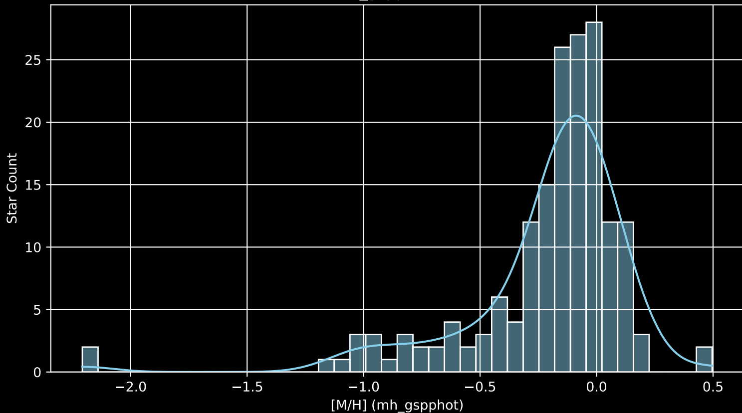
APOGEE DR17 Field: [191-04 [M/H] (mh_gspphot) (n= 174)
